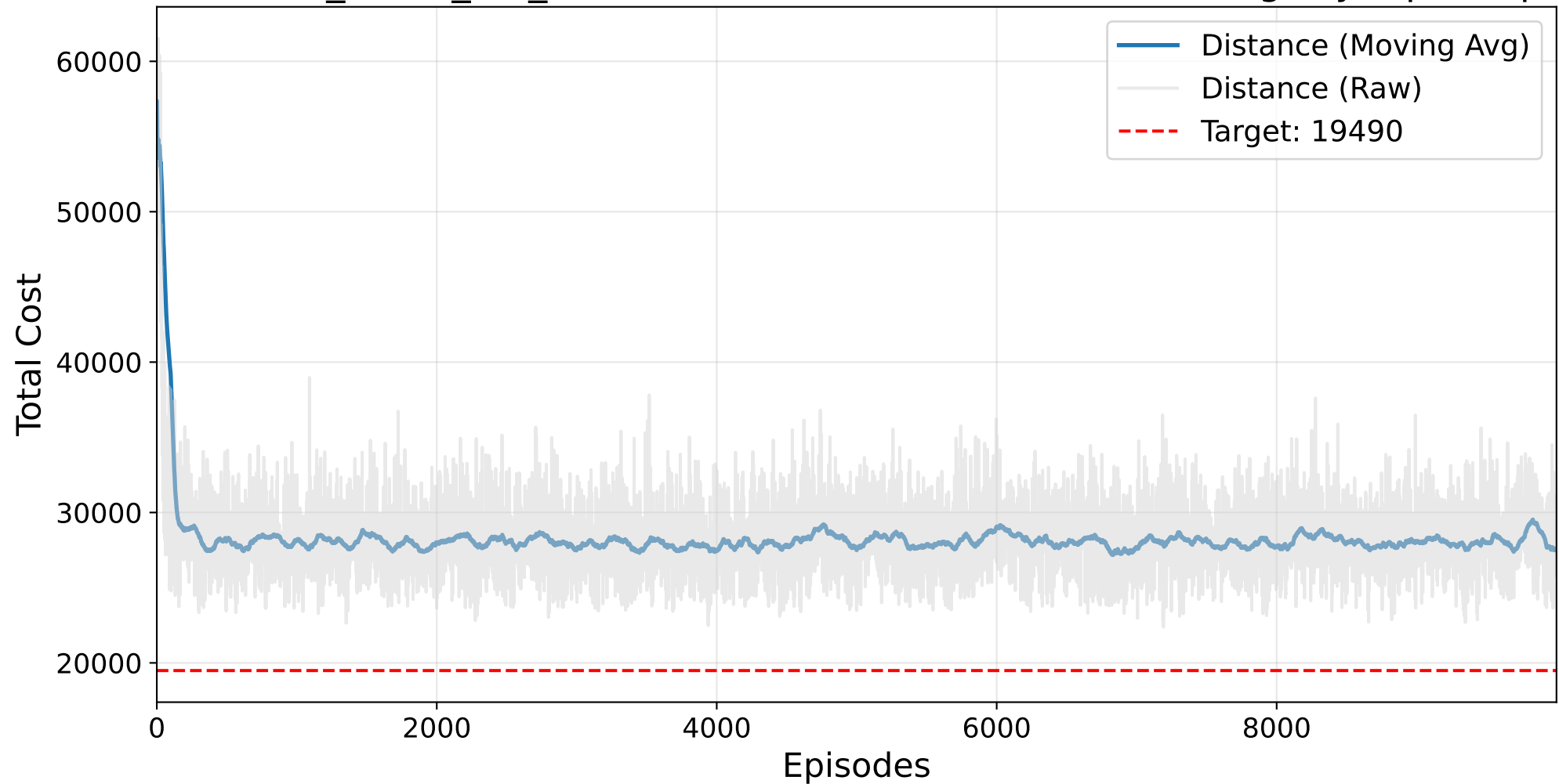
Final NO_MASK_NO_BAYESIAN Masked AutoRL-SOP Training - ry48p.3.sop
